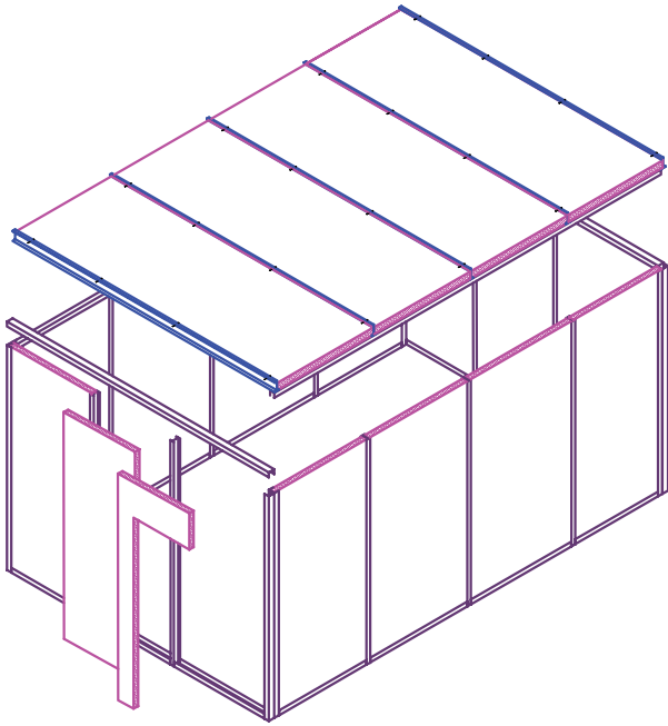
Exploded View: Typical Durra DIY Studio Kit
